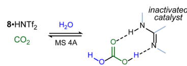
Figure 2. Catalyst Inactivation Pathway and Its Recovery Using MS 4A.
